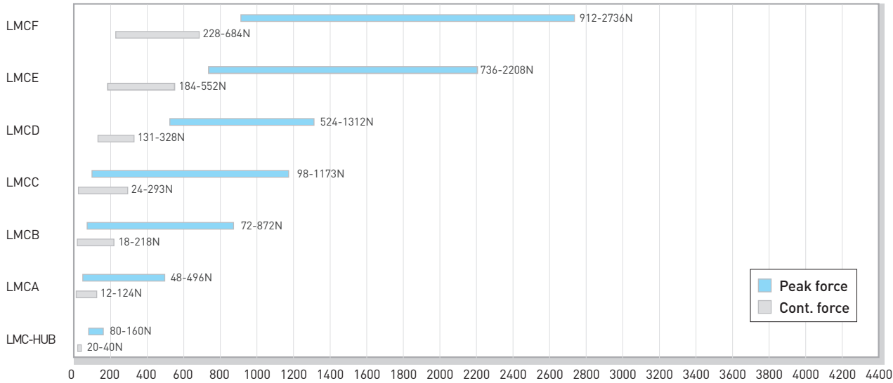
Force chart for LMC series
